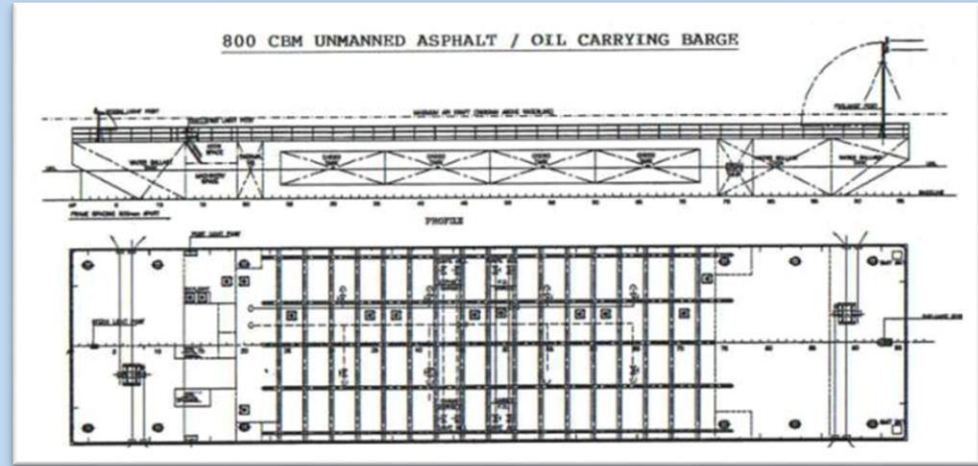
800 CBM UNMANNED ASPHALT / OIL-CARRYING BARGE
