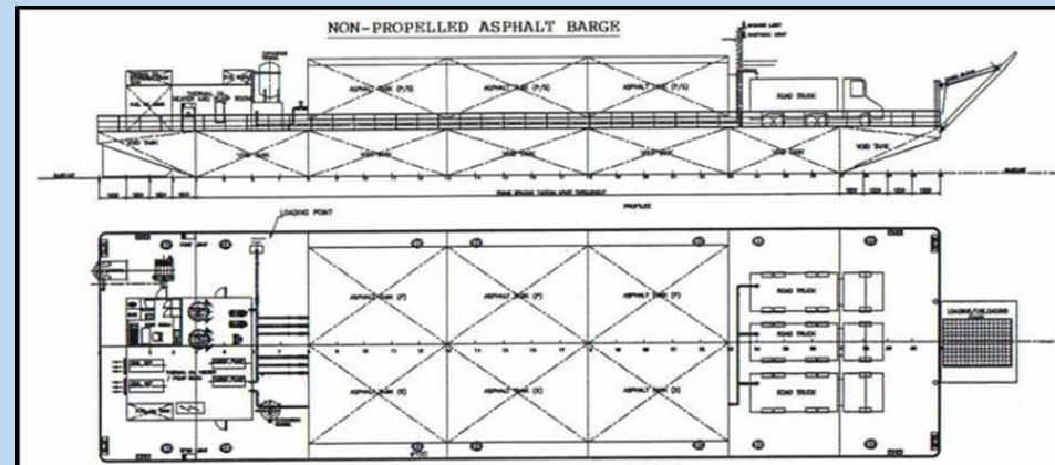
NON-PROPELLED ASPHALT BARGE
